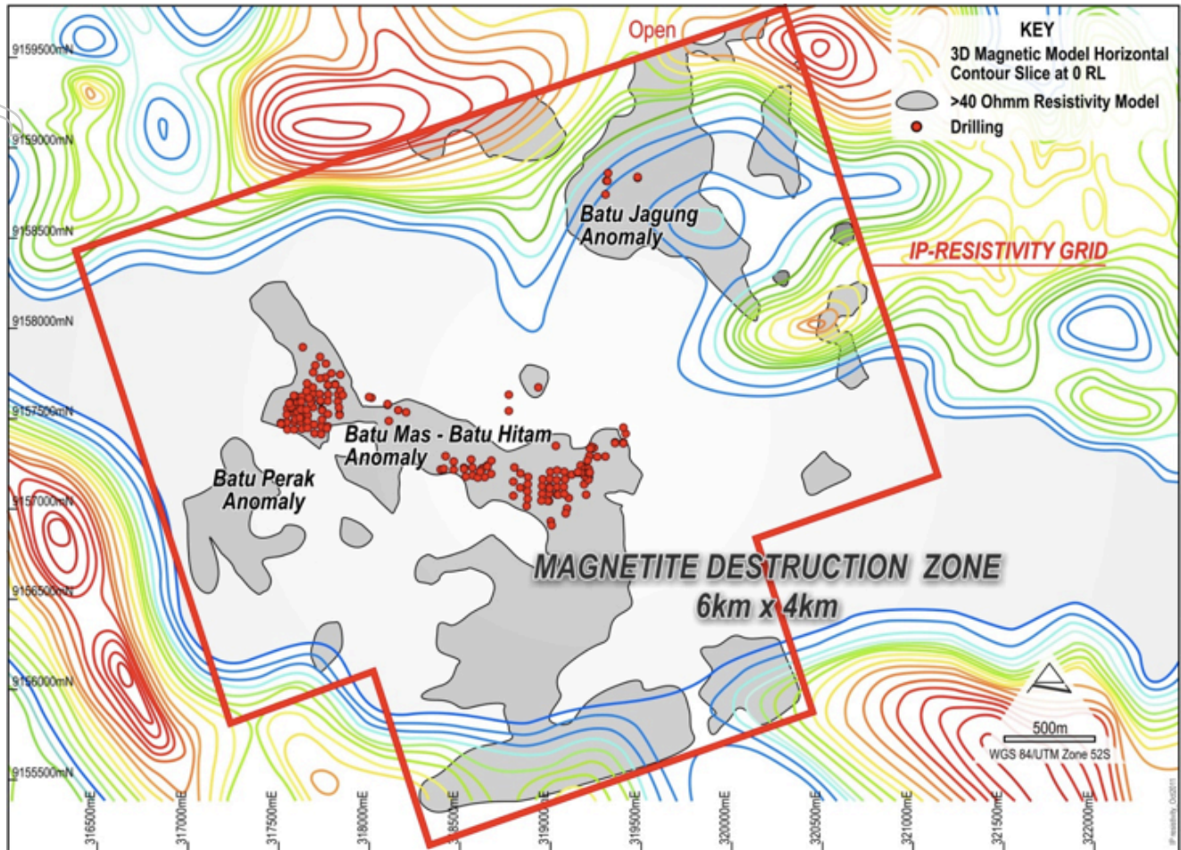
Figure 1: Lakuwahi Project – Extended 3D IP-Resistivity Grid with Results
