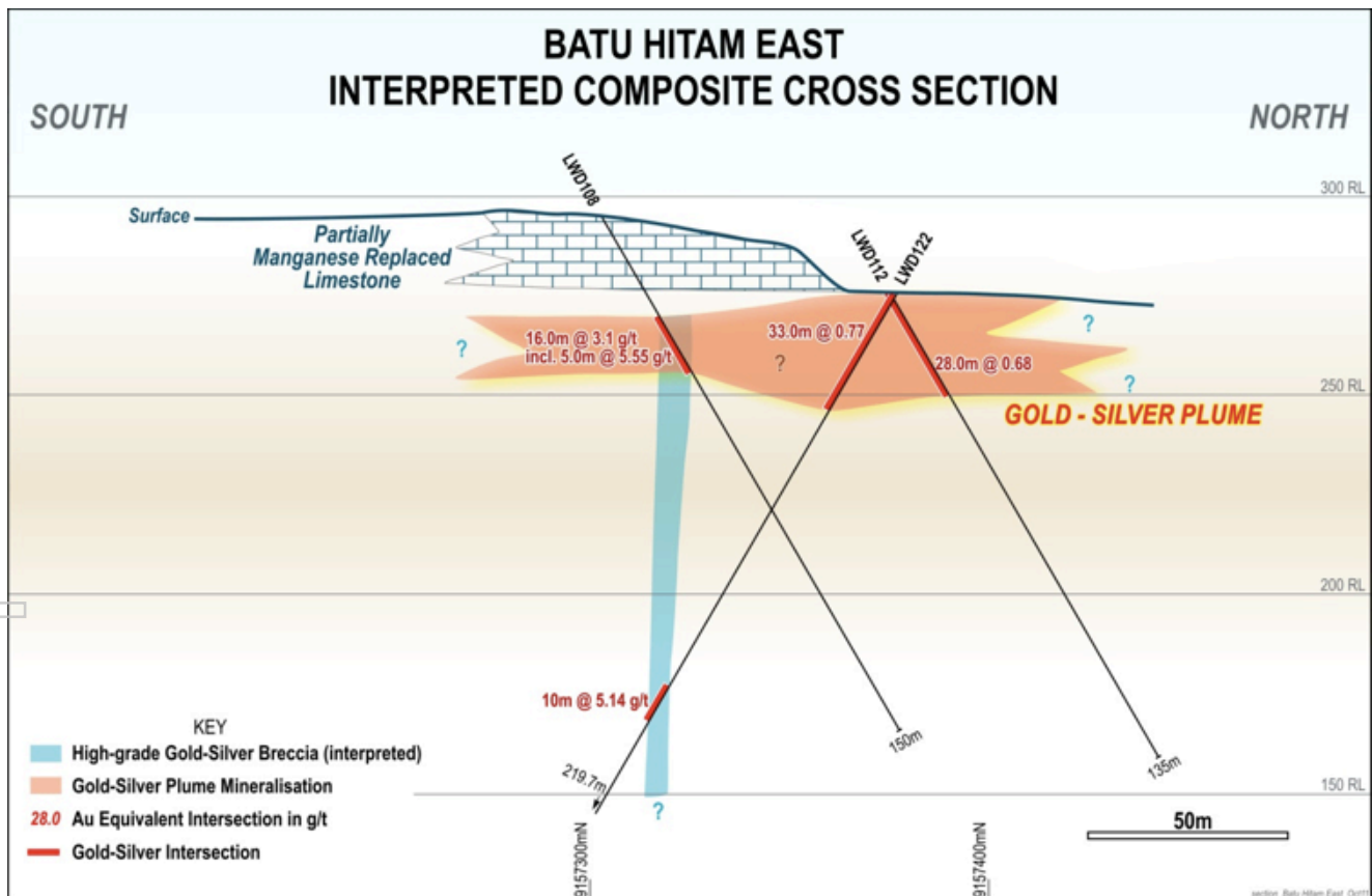
Figure 2: Lakuwahi Project, Batu Hitam East – Interpreted Cross Section
